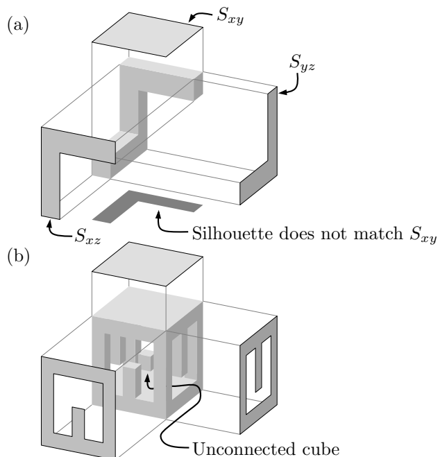
Figure 1: (a) An invalid trip-let: the z -silhouette does not match the top shape. (b) A non-connected trip-let: it consists of two components.
